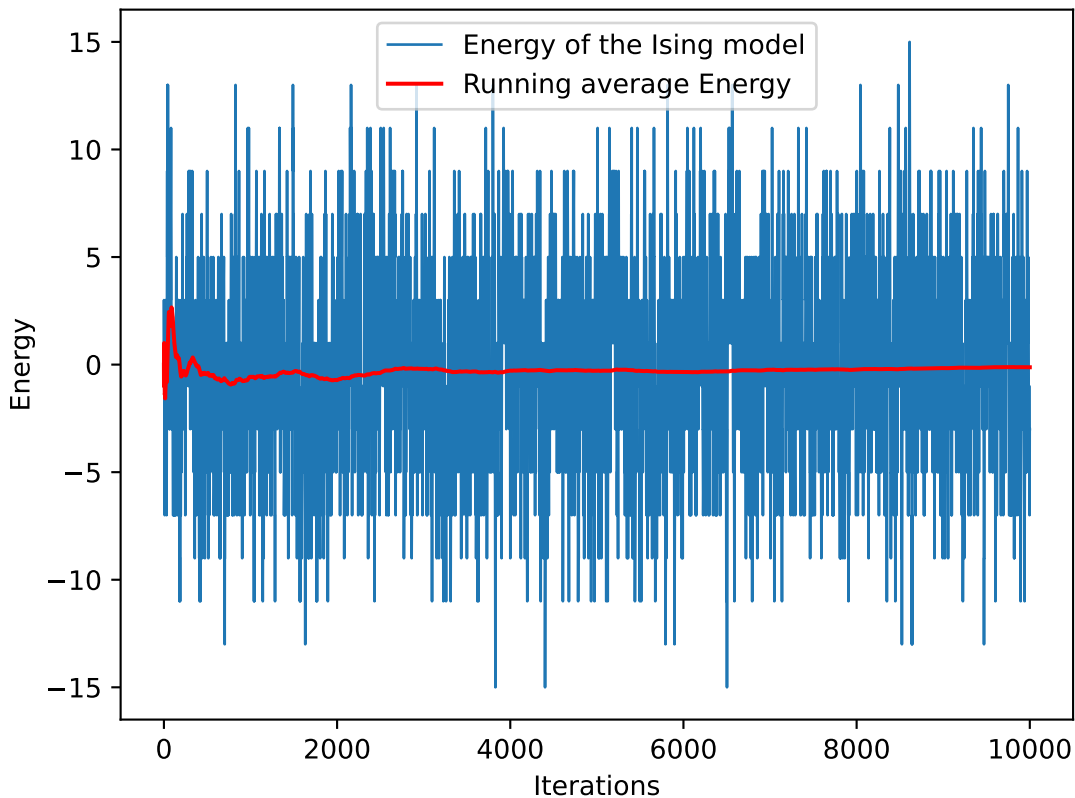
Evolution of a stochastic simulation of the 1D Ising model, at \beta = 0 J = 1 h = 0
